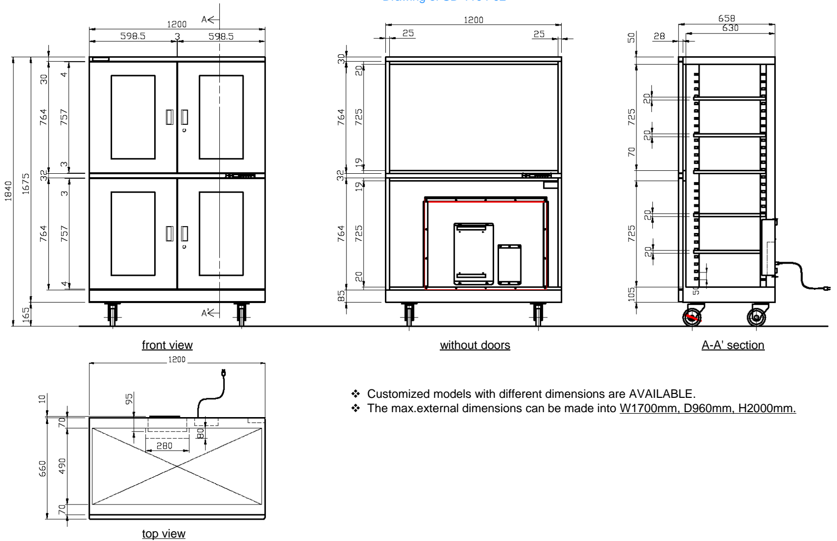
Drawing of SD-1104-02
